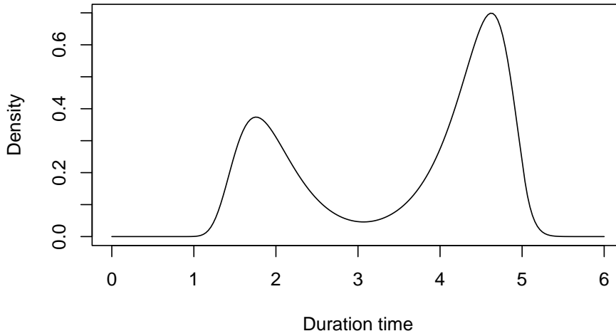
Figure 2: Old Faithful Geysers. Estimated density for duration time obtained from an unconditional transformation model where the transformation function was parameterised as a Bernstein polynomial of order eight. The plot reproduces Figure 1 (right panel) in Hothorn et al. (2017) .
