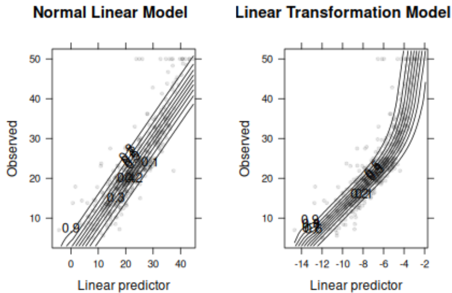
Figure 7: Boston Housing. Predicted vs. observed for the normal linear model (left) and the linear transformation model with smooth baseline transformation (right). The observations are overlaid with the conditional quantiles of the response given the linear predictor.
