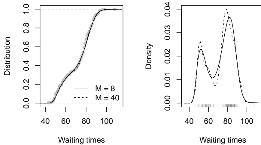
Figure 3: Old Faithful Geysers. Estimated distribution (left, also featuring the empirical cumulative distribution function as grey circles) and density (right) function for two transformation models parameterised in terms of Bernstein polynomials of order eight and 40. The right plot reproduces the density for M = 8 shown in Figure 1 (left panel) in Hothorn et al. (2017) .
