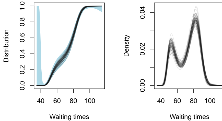
Figure 15: Old Faithful Geysers. Model-based bootstrap for distribution (left, the blue area depicts the asymptotic confidence band from Figure 14) and density (right) function for the unconditional transformation model parameterised in terms of a Bernstein polynomials of order 8.
